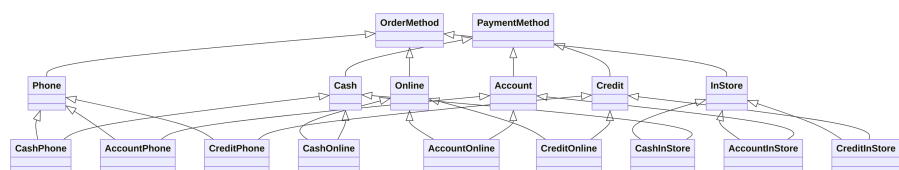
Figure 10.26 Mermaid Class Diagram using ELK layout engine
