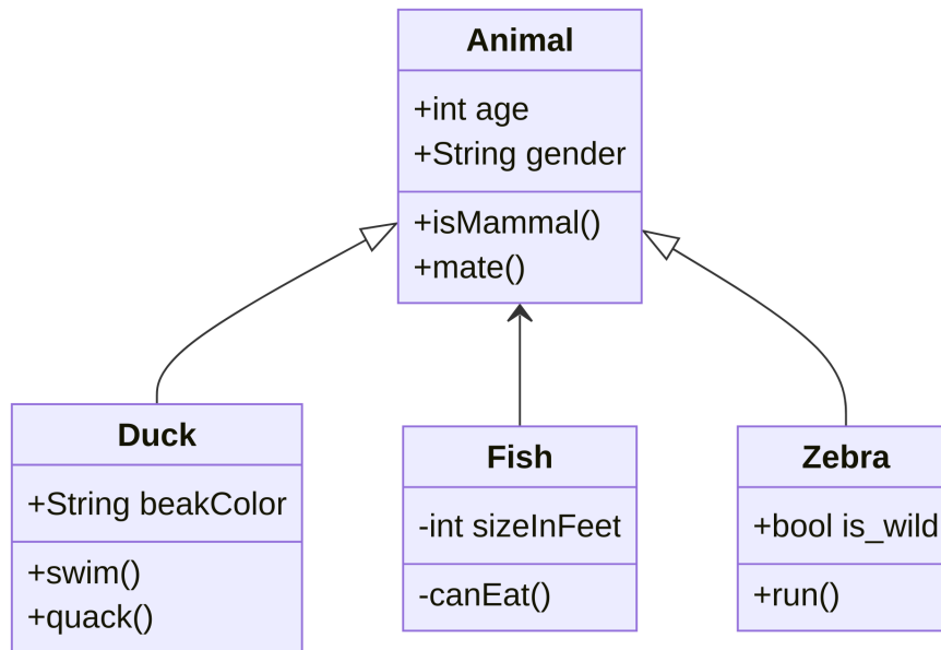
Figure 10.24 Mermaid Class Diagram
