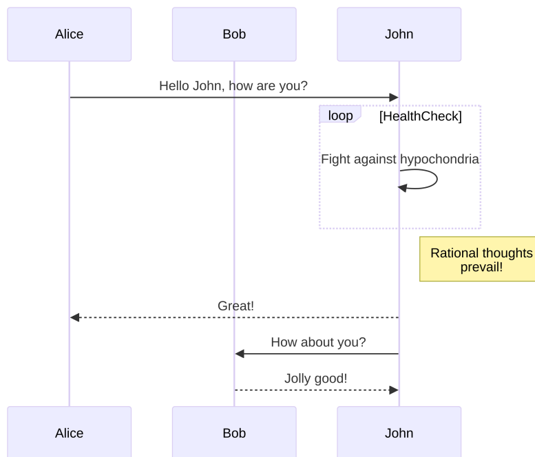
Figure 10.25 Mermaid Sequence Diagram
