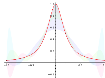
Figure 10.31 Sage polynomial approximations of f(x) = 1/(1 + 25x^2)
