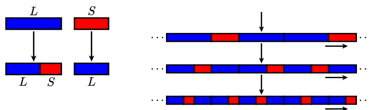
Figure 10.6 Fibonacci tilings are one-dimensional analogs of Penrose tilings. The diagram on the left introduces the process of deflation that is used to produce tilings while the diagram on the right explains why they are aperiodic.
