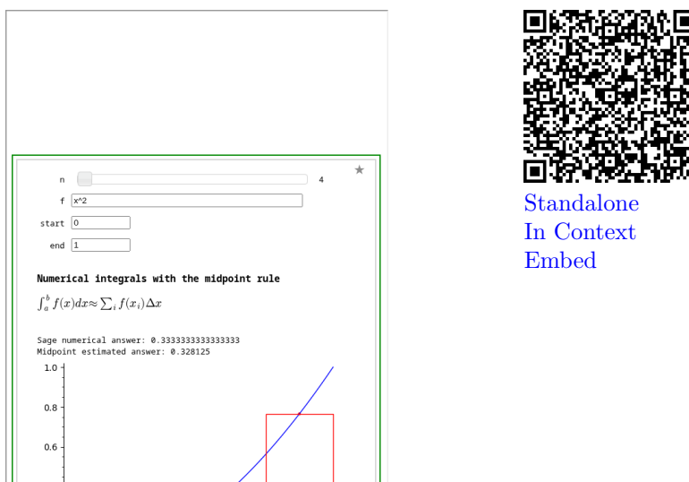
Figure 14.21 Numerical integrals using the midpoint rule
